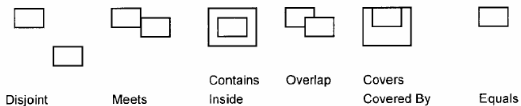
Figure 2.5b Topological Relations
