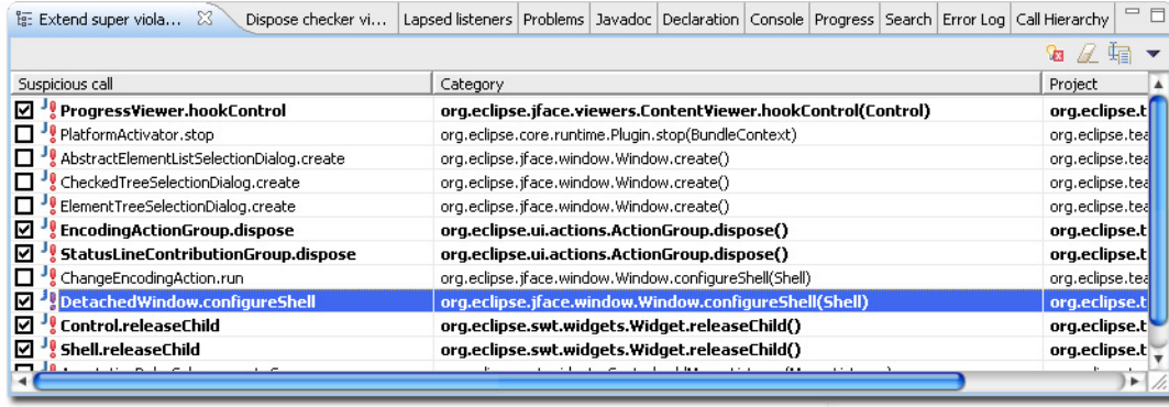
Figure 1: Output of the extend super rule checker. Confirmed potential violations are shows in bold.
