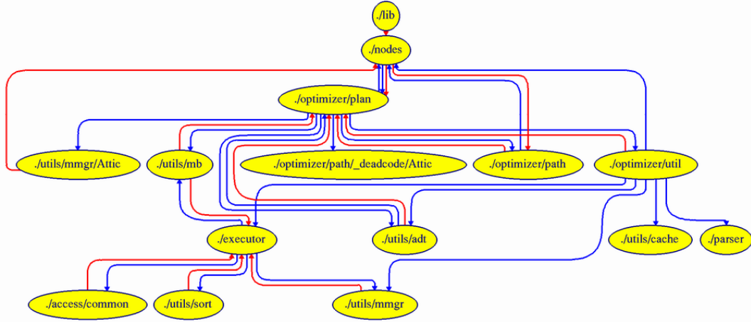
Figure 5: High-Level (Subsystem) Call Graph for Postgres Optimizations
