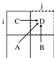
Figure 3. Calculation pattern for cell (i, j) .
